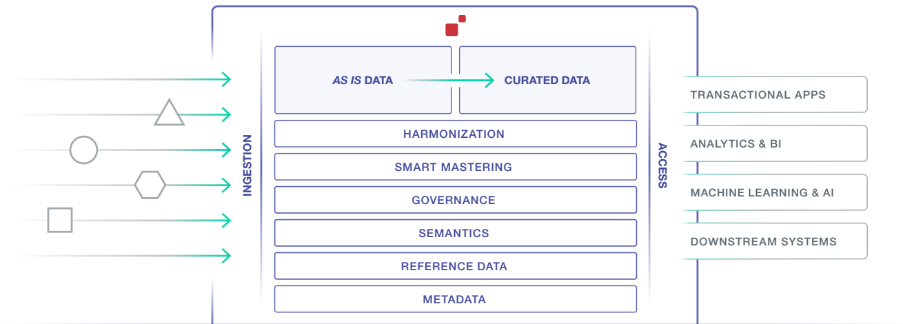
The MarkLogic Data Hub Platform
